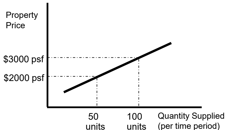
Supply Curve
