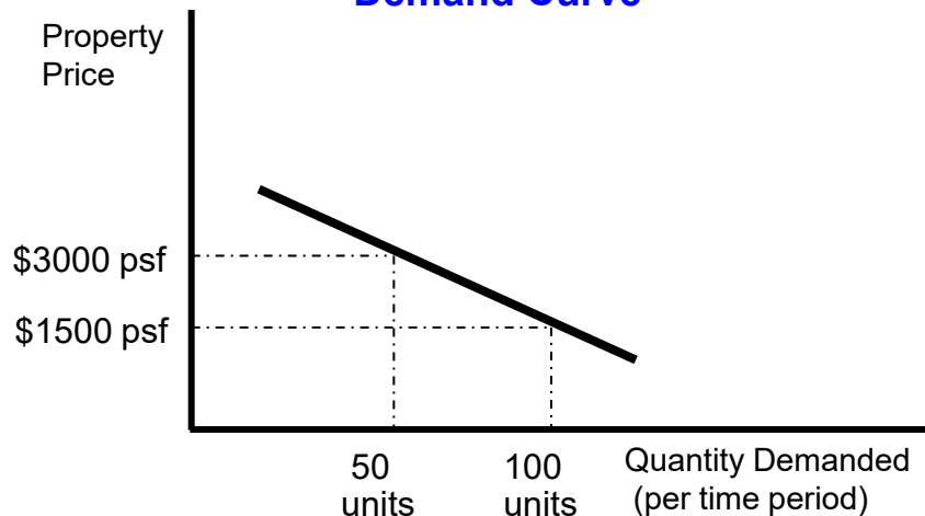
Demand Curve
